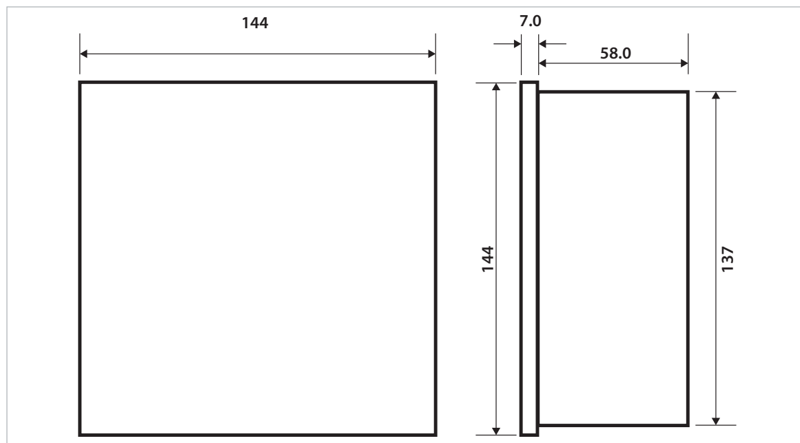
Figura 2.8: Dimensions
