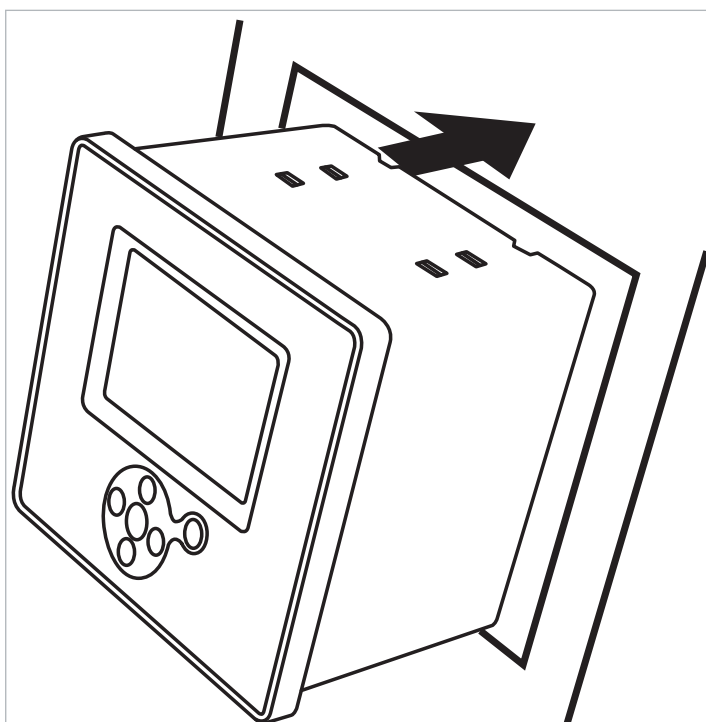
Figura 2.1: Placing PFW03-M on the Panel
