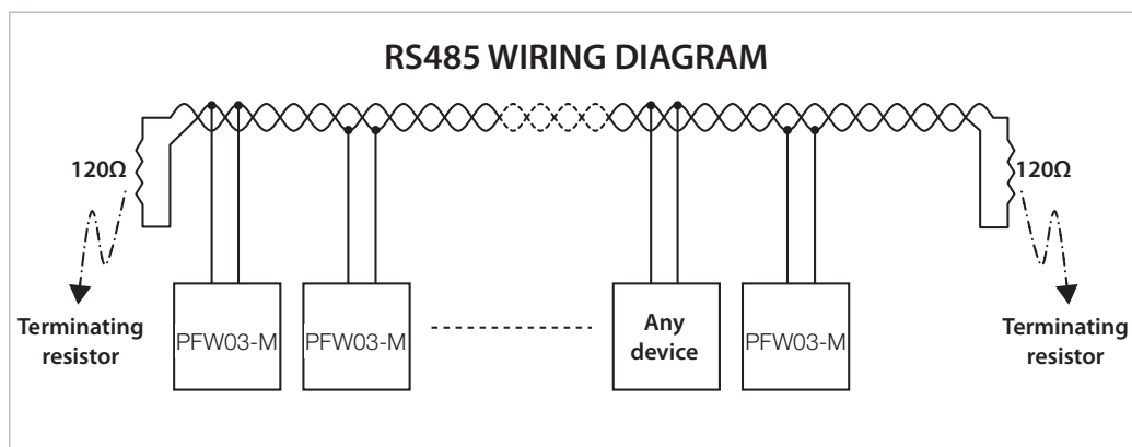
Figura 4.1: RS485 Wiring Diagram
