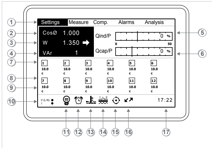
Figura 1.1: PFW03-M12
