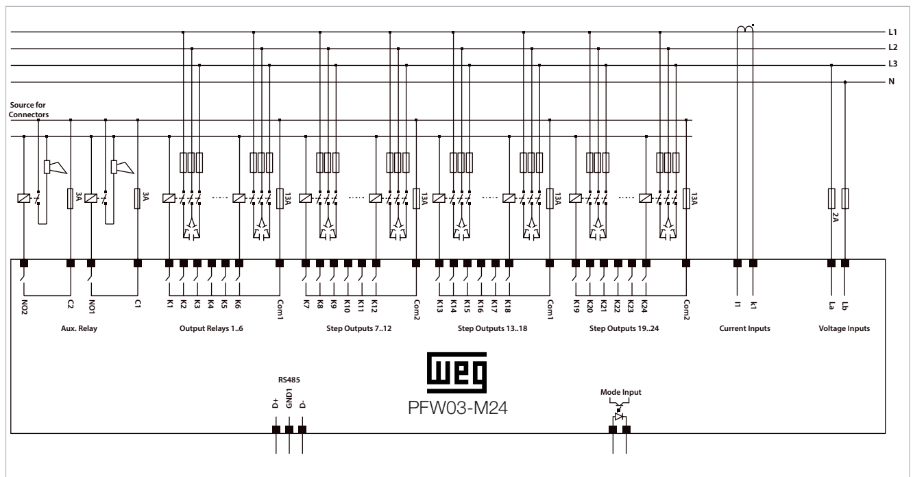
Figura 2.7: PFW03-M Connection Diagram (24 Steps)
