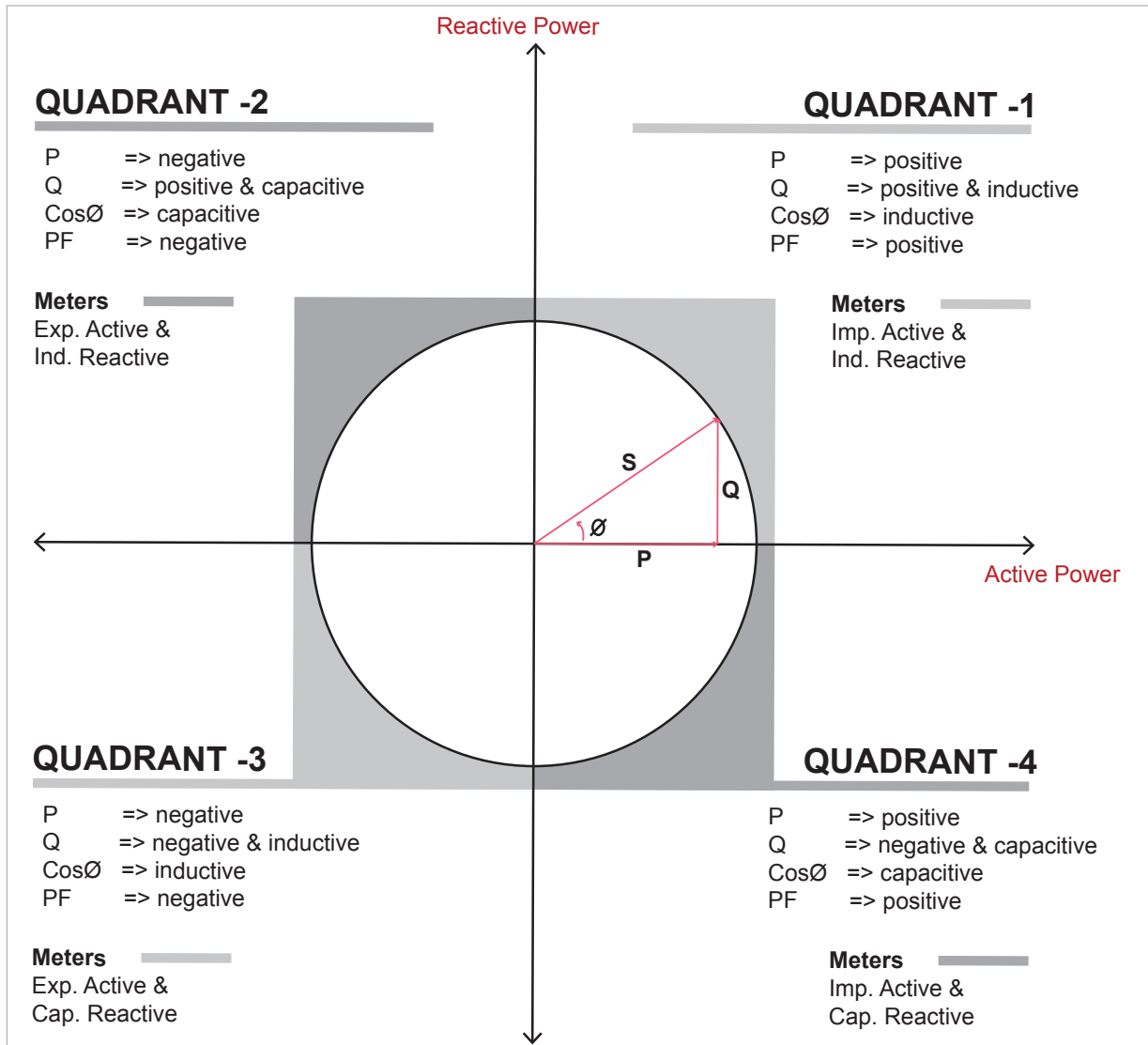
Figura 1.5: Four-Quadrant Representation
