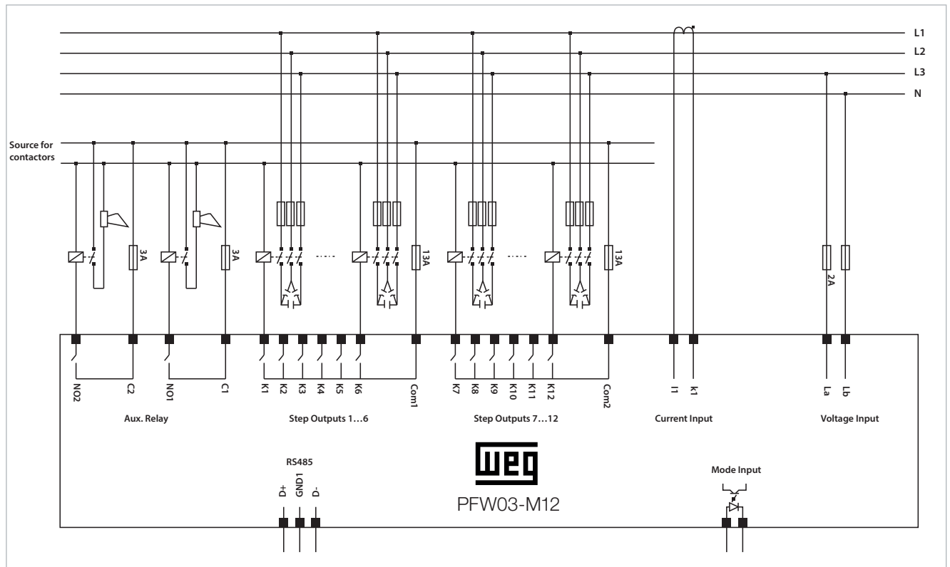
Figura 2.6: PFW03-M Connection Diagram (12 Steps)
